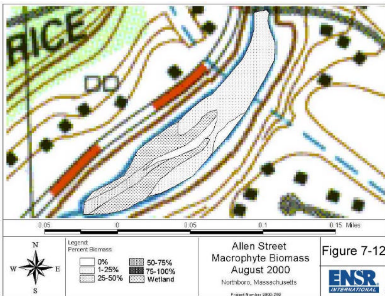
Figure 7-19 Allen Street Macrophyte Biomass, August 2000
