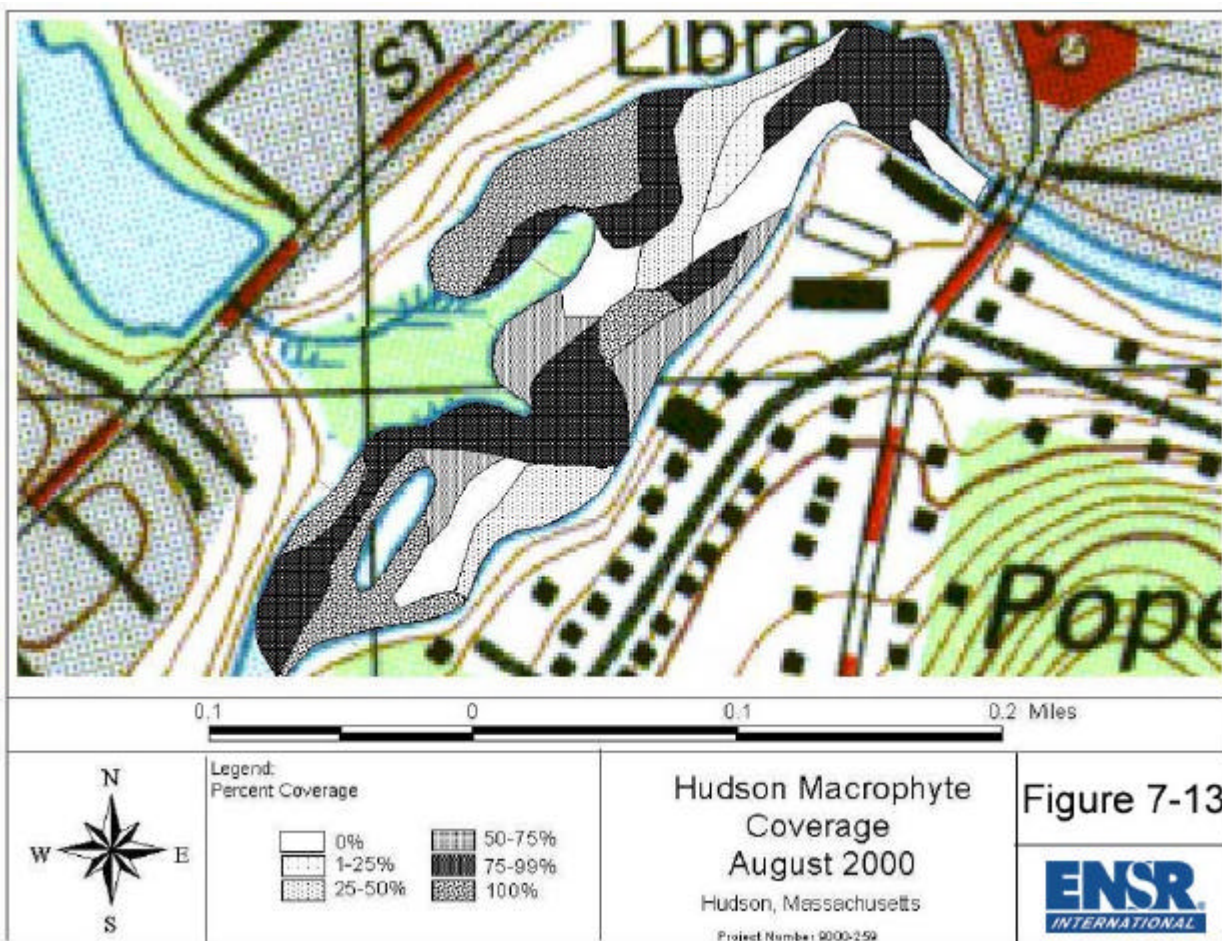
Figure 7-20 Hudson Macrophyte Coverage, August 2000
