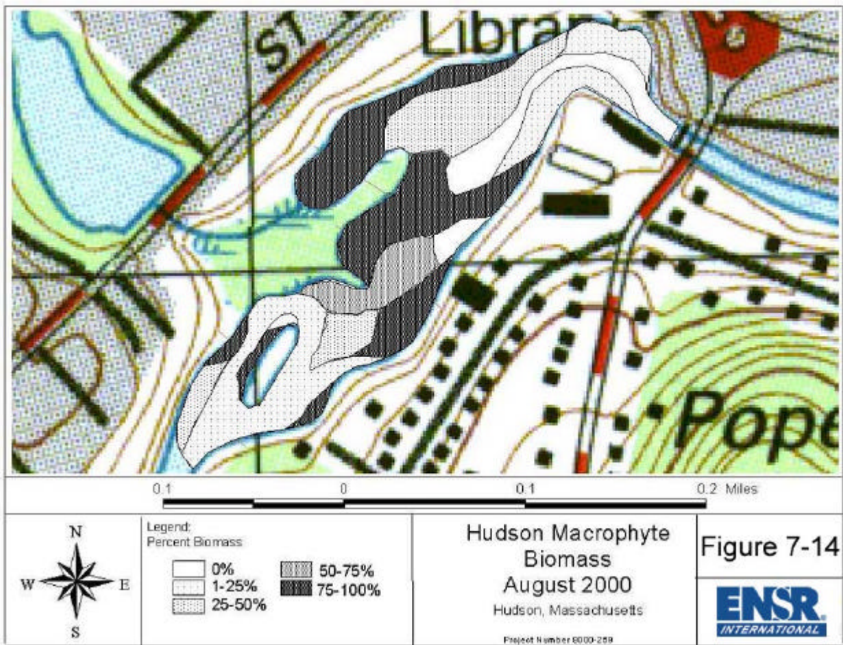
Figure 7-21 Hudson Macrophyte Biomass, August 2000
